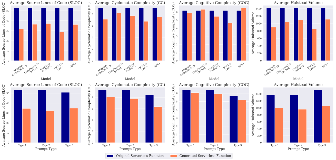
Fig. 5: Code Quality Metrics of Original and Generated Functions per Model (first row), per Prompt Type (second row)
