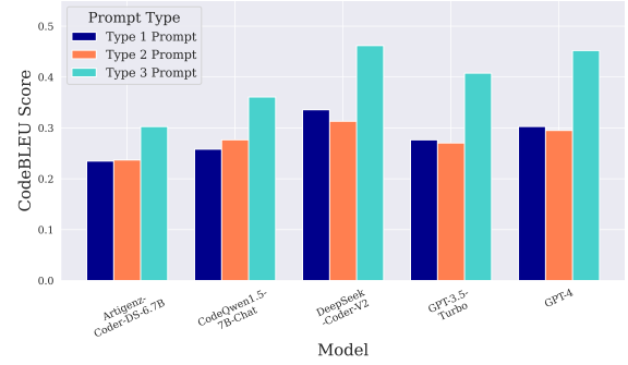
Fig. 4: Avg. CodeBLEU Scores for Generated Functions per Model and Prompt Type
