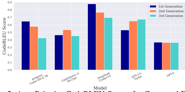
Fig. 2: Avg. Pairwise CodeBLEU Scores for Generated Functions per Model
